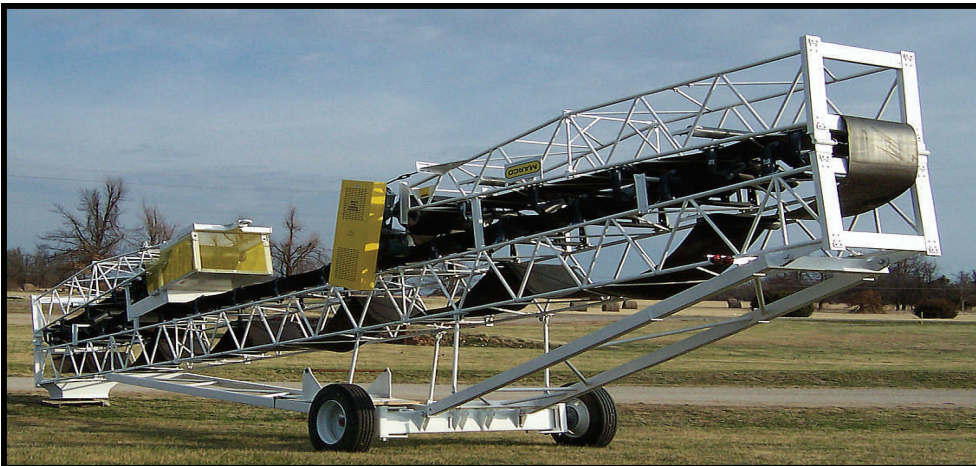
MARCO RADIAL STACKER CONVEYOR
